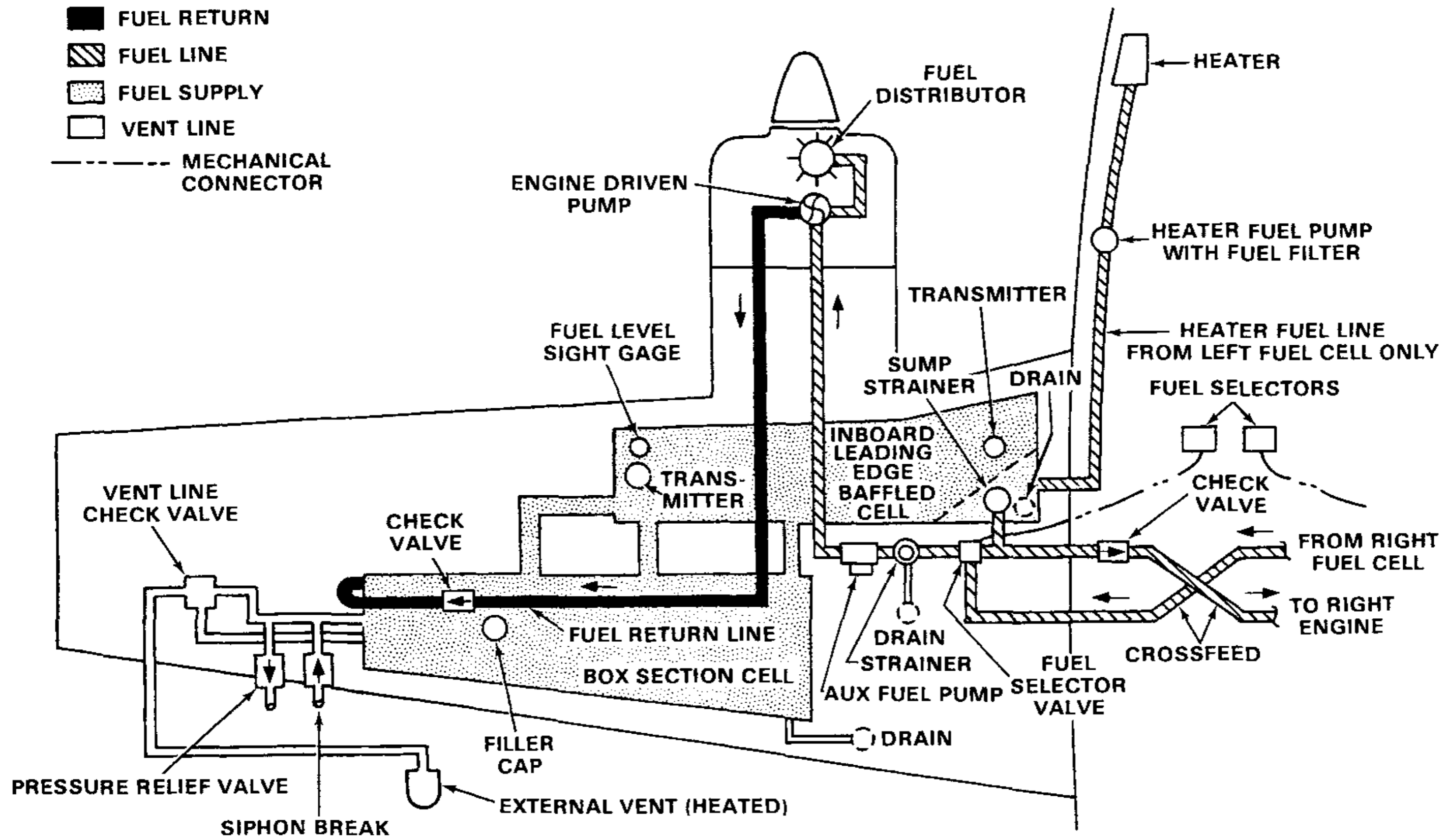
FUEL SYSTEM SCHEMATIC
