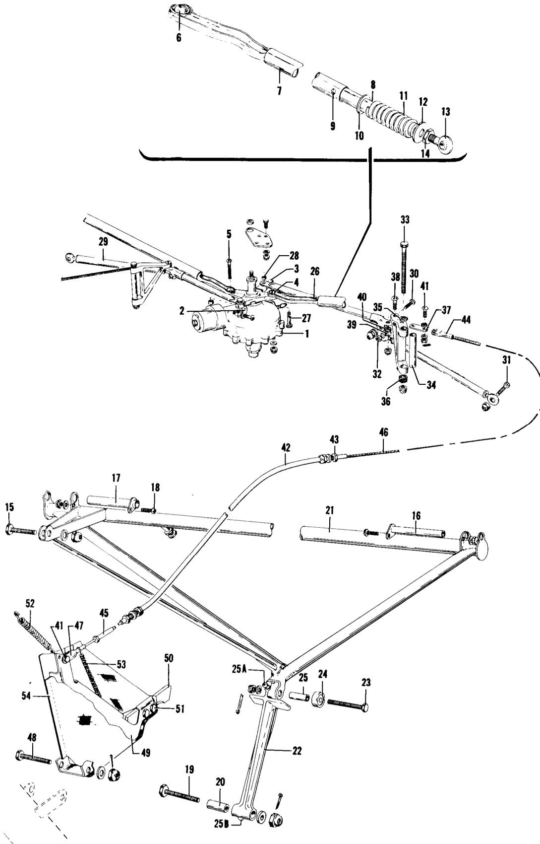
Figure 35. Main Landing Gear Retract Installation
