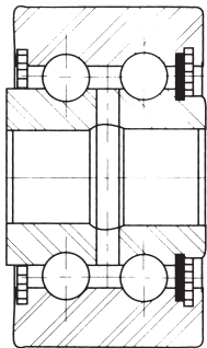
Crane Trolley: Ball bearing design provides axial load capability.
