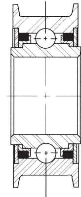
Textile Loom: Integral idler pulley and positive sealing economical replacement.
