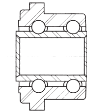
Coin Changer: Double row design with soft races to allow the bearing to be staked in place.
