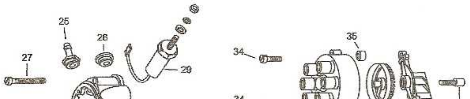
6300 SERIES MAGNETO
